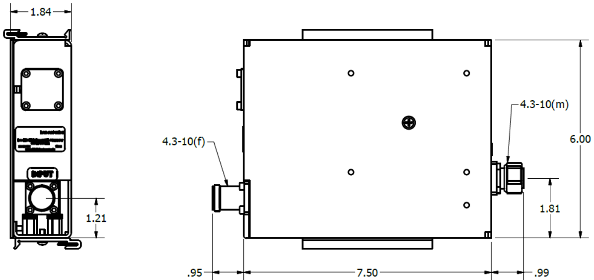
OUTLINE DRAWING
