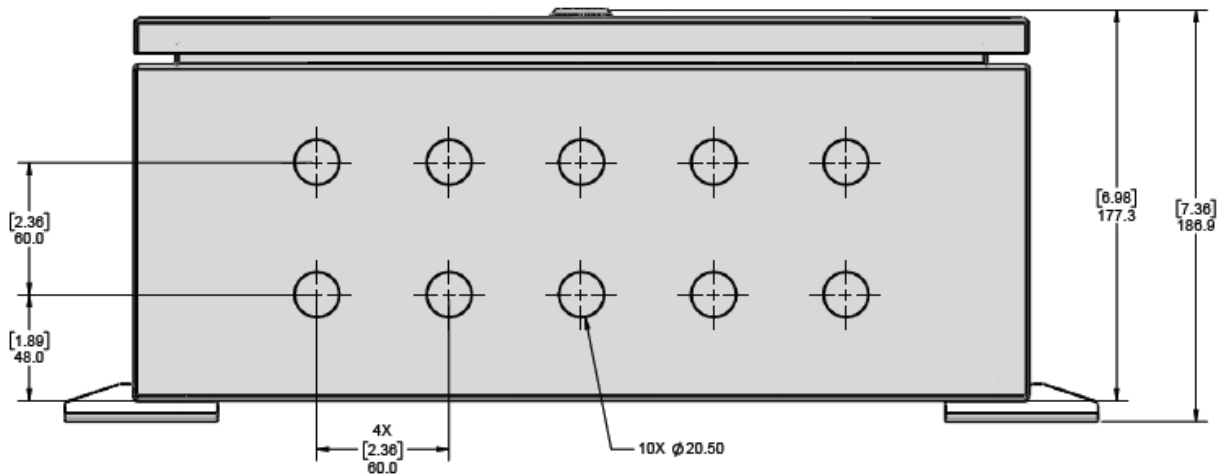
OUTLINE DRAWING
