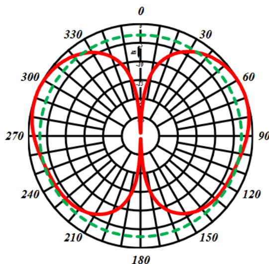
Vertical Pattern
