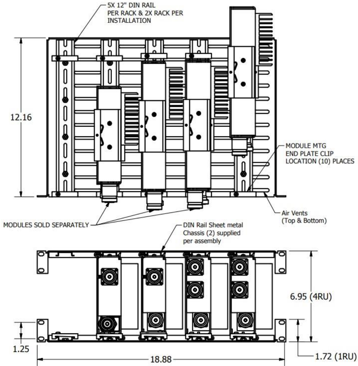
ATTENUATOR TRAY ASSEMBLY 80-0939
