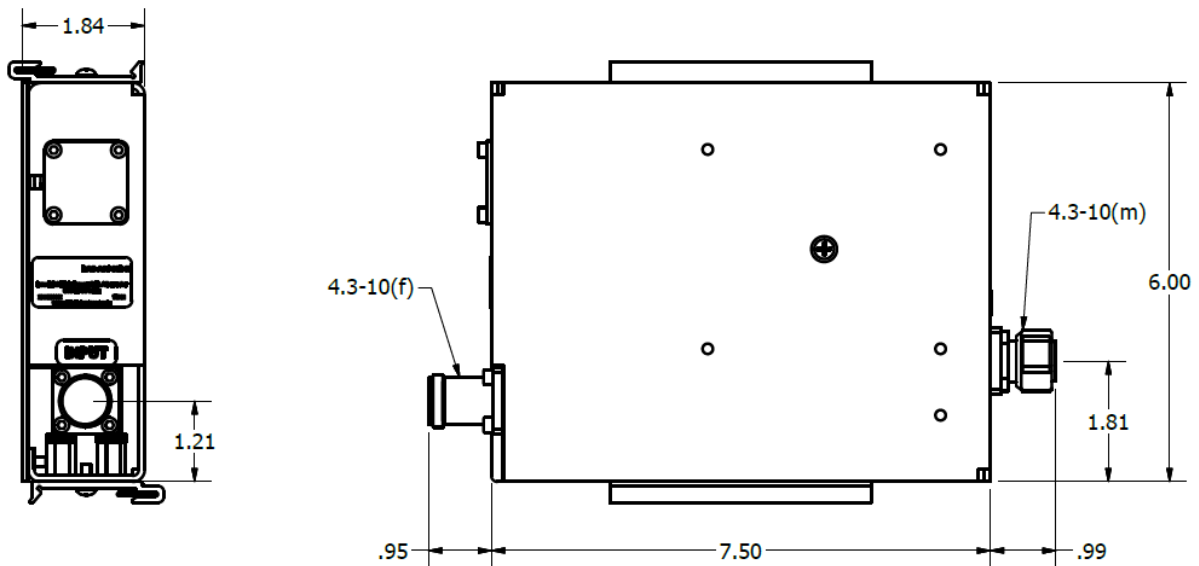
OUTLINE DRAWING
