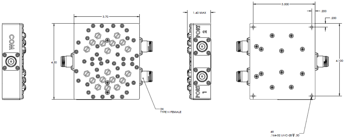
OUTLINE DRAWING
