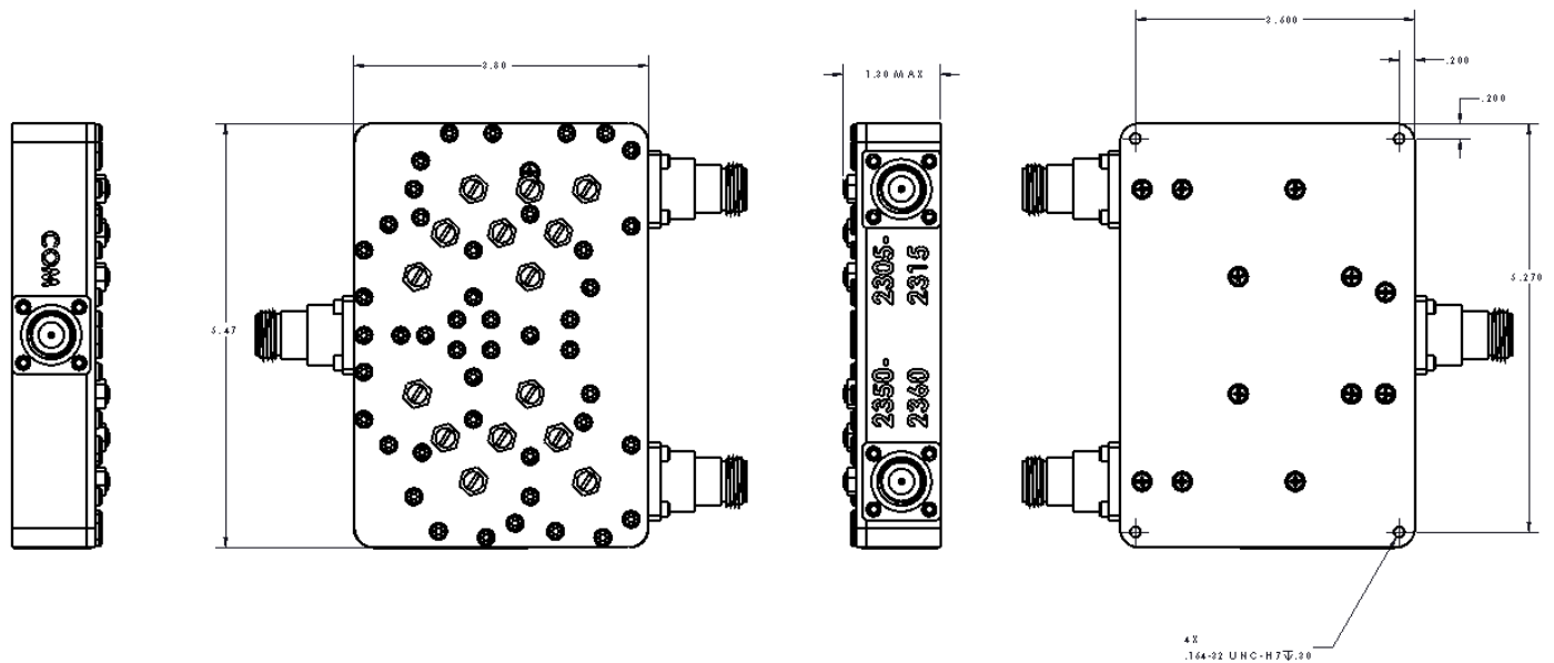
OUTLINE DRAWING
