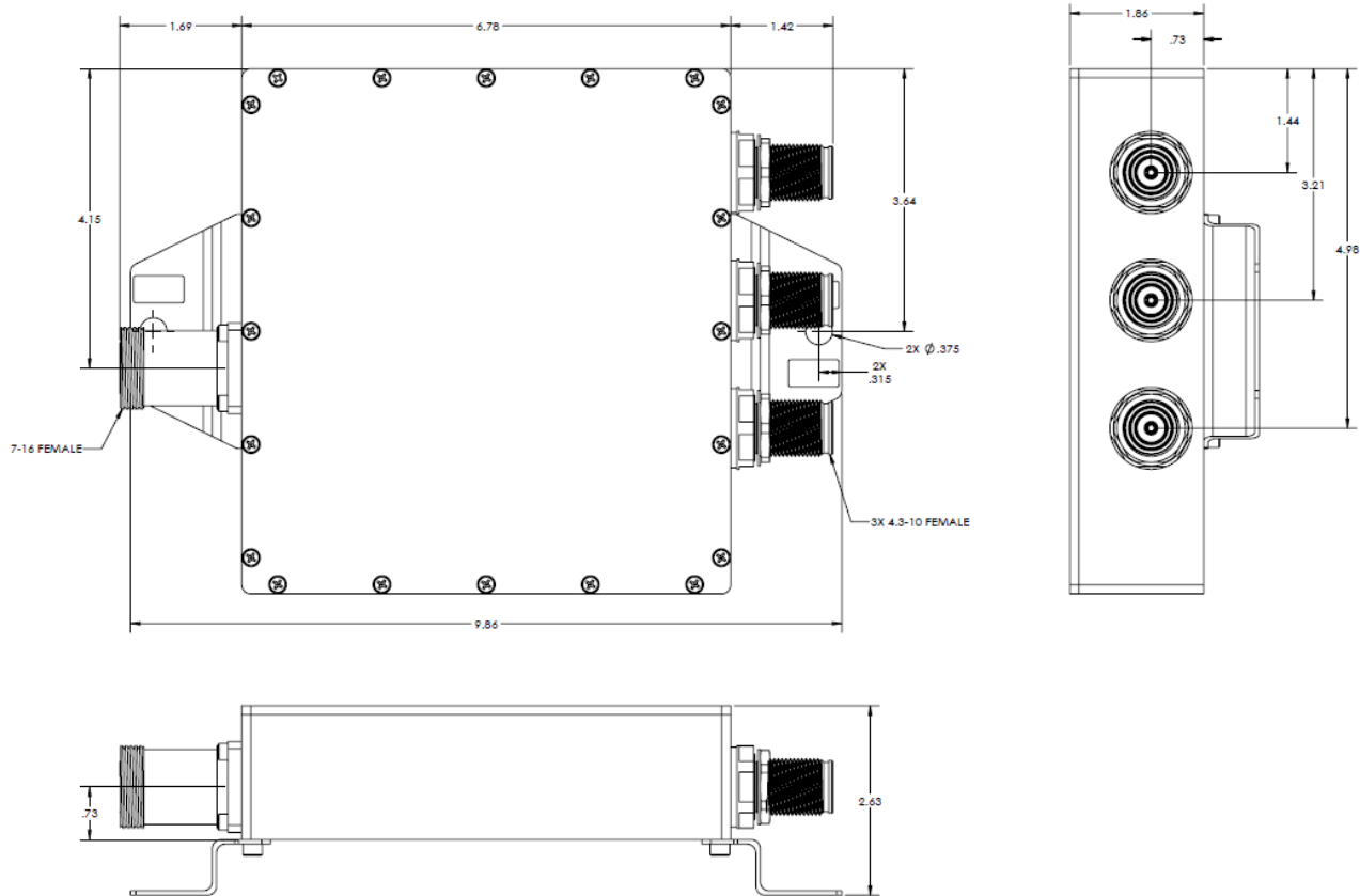
OUTLINE DRAWING
