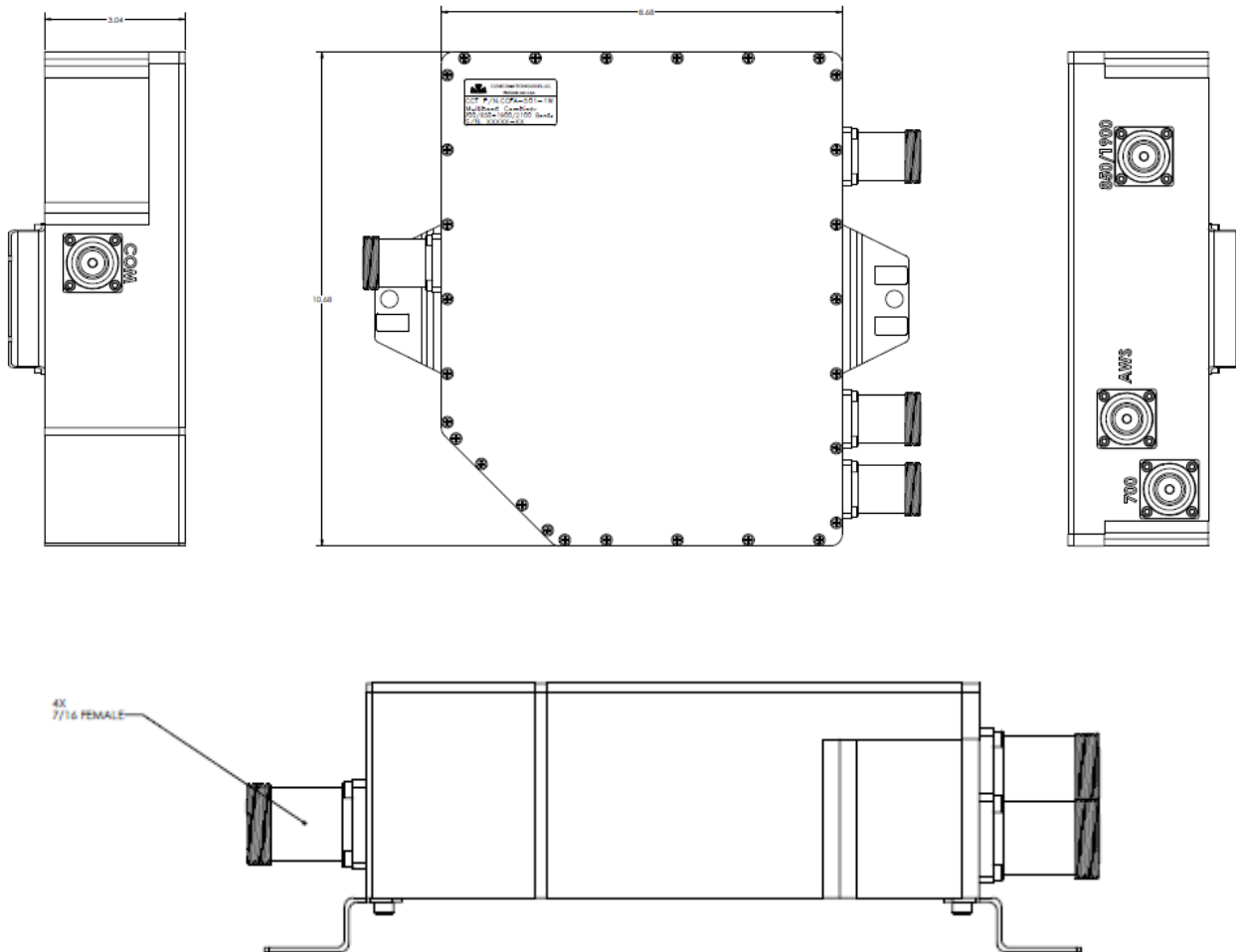
OUTLINE DRAWING
