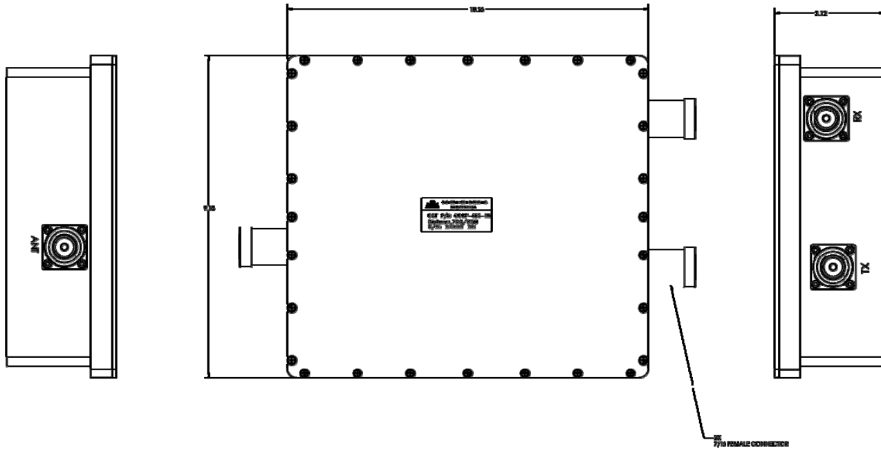
OUTLINE DRAWING
